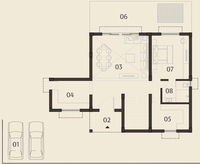
1 BHK Area: 179 SQ.YD. GROUND FLOOR PLAN
