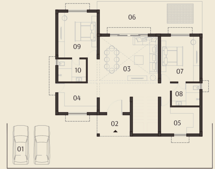
3 BHK Area: 283 SQ.YD. GROUND FLOOR PLAN
