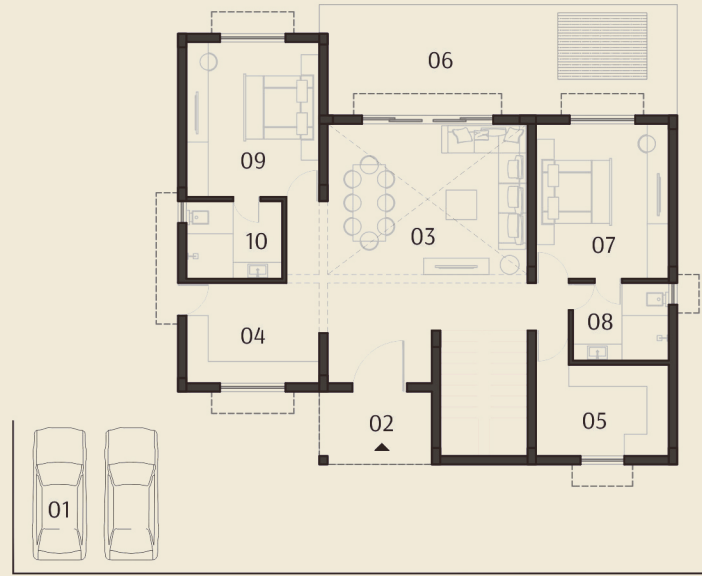
2 BHK Area: 225 SQ.YD. GROUND FLOOR PLAN
